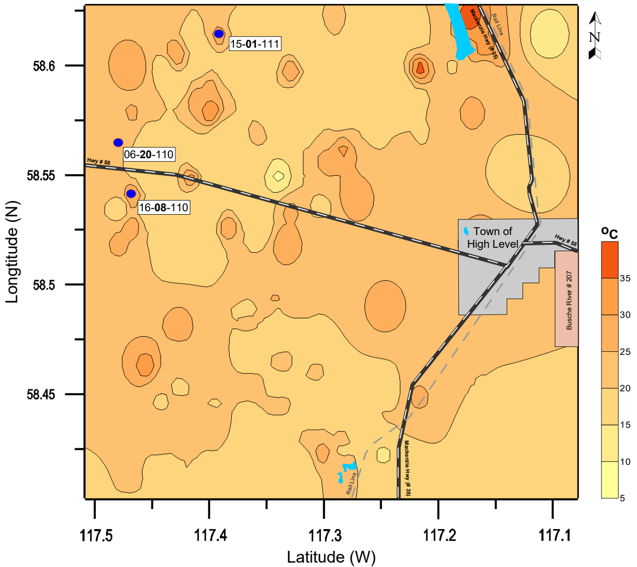
Bottom-Hole Temperature Map (at Depths Less than 350m - Town of High Level)
