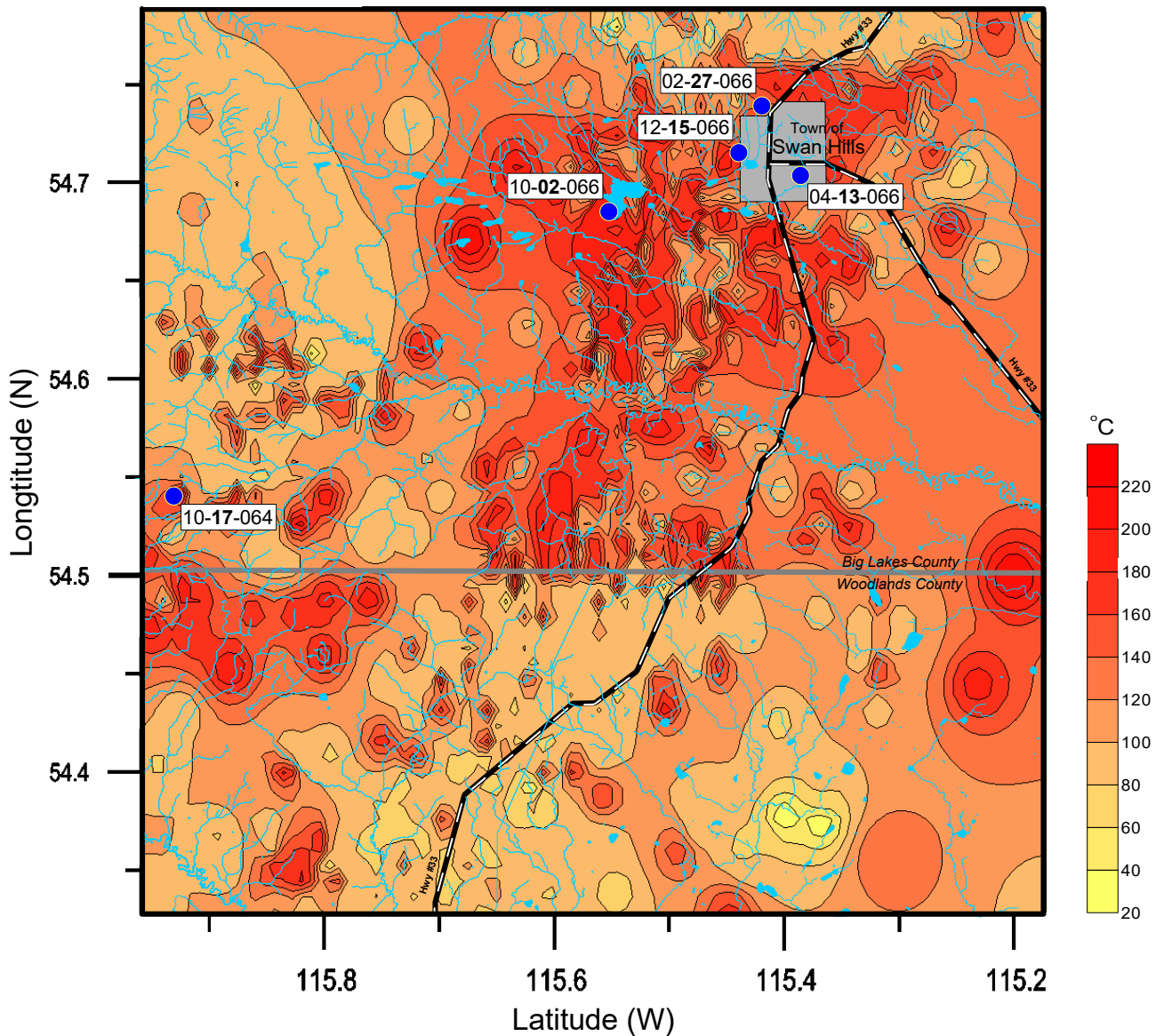
Corrected Bottom-Hole Temperature Map (at Depths Greater than 2.5km - Town of Swan Hills)
