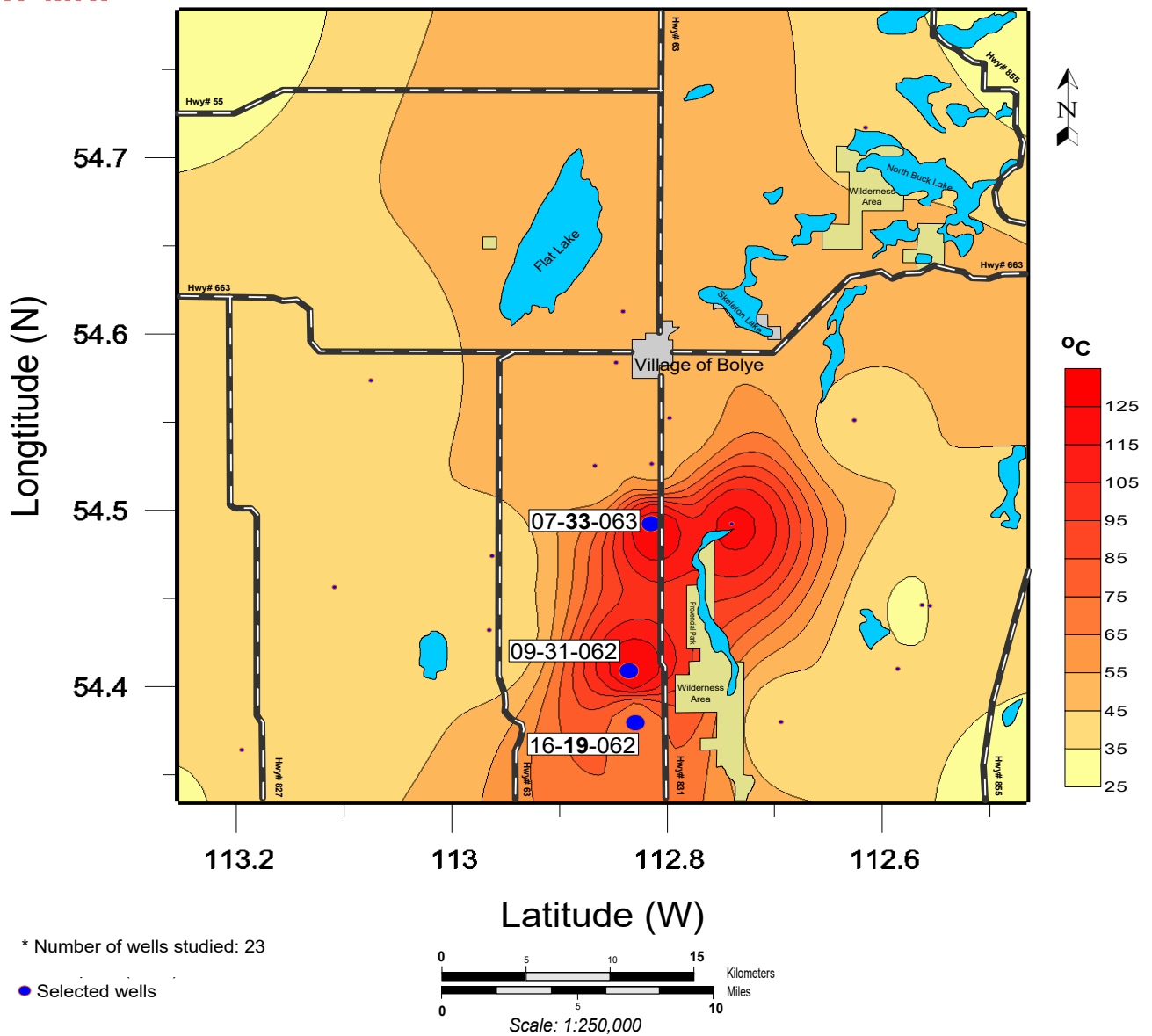
Corrected Bottom-Hole Temperature Map (at Depths Greater than 0.9km - Athabasca County)
