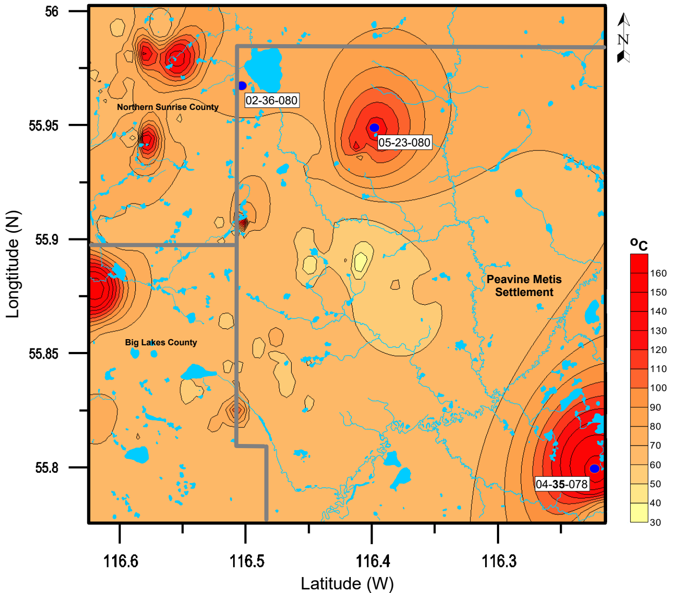
Corrected Bottom-Hole Temperature Map (at Depths Greater than 2.5km - eastern Peavine Metis Settlement )
