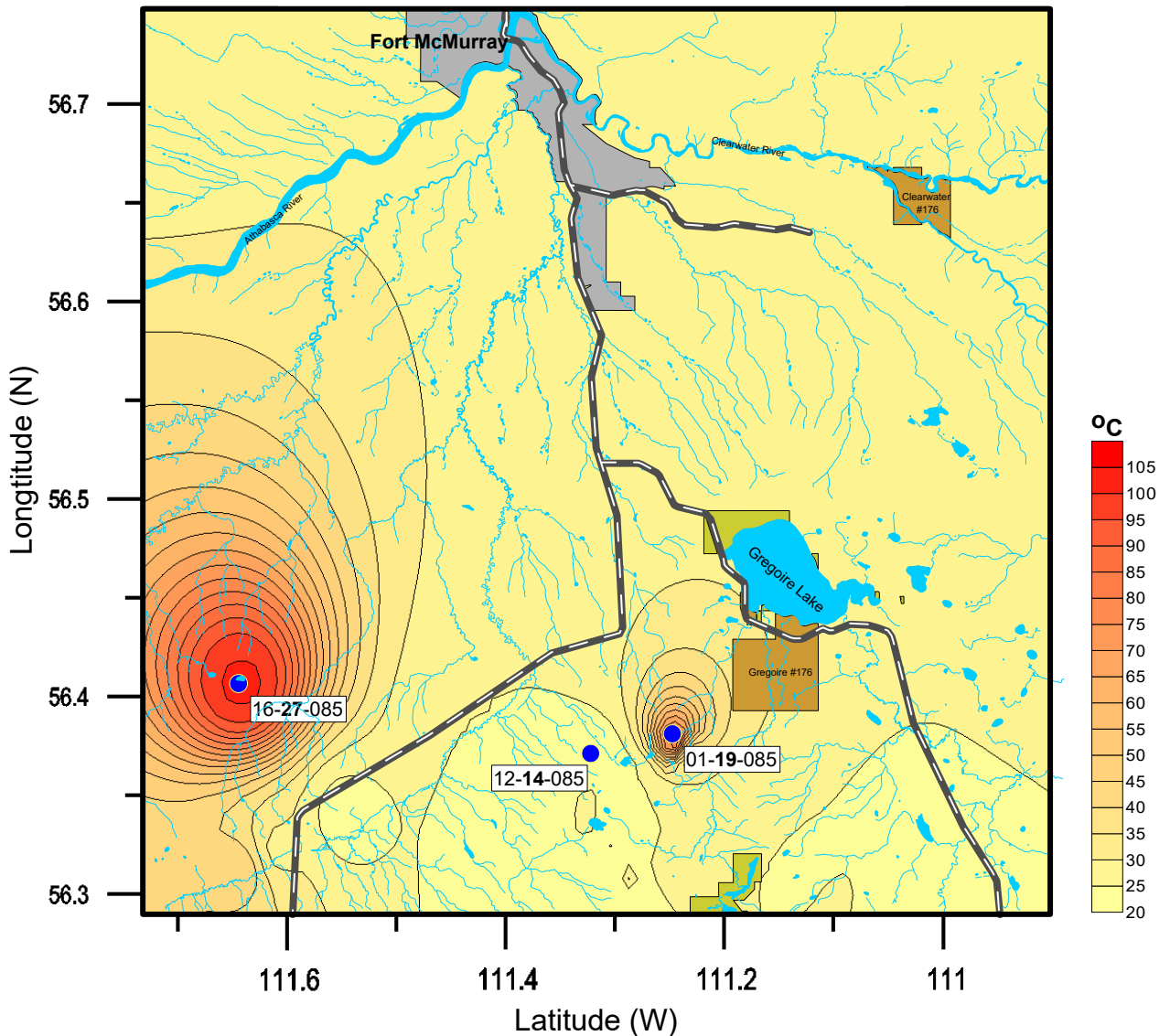
Corrected Bottom-Hole Temperature Map (at Depths Greater than 0.5km - Wood Buffalo)
