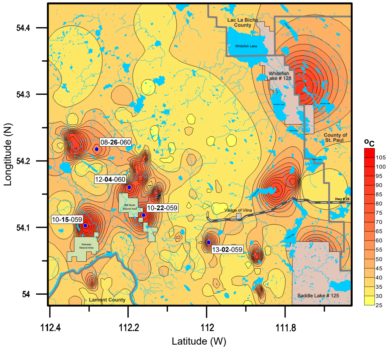
Corrected Bottom-Hole Temperature Map (at Depths Greater than 0.7km - Smoky Lake County)
