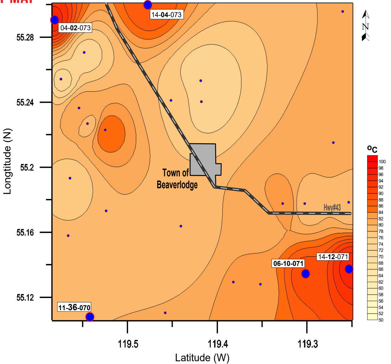
Corrected Bottom-Hole Temperature Map (at Depths Greater than 2.5km - Town of Beaverlodge)
