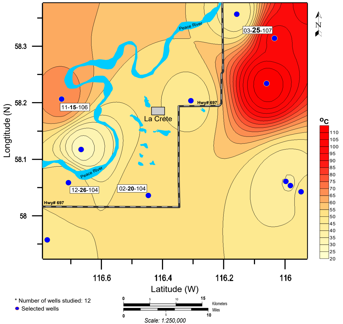
Corrected Bottom-Hole Temperature Map (at Depths Greater than 1km - Mackenzie County)
